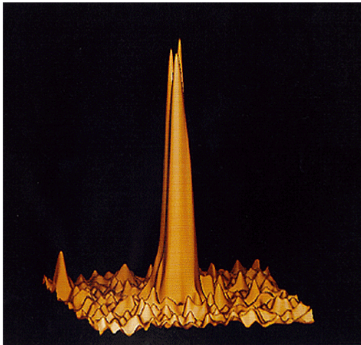
3-D representation of Rosat image
