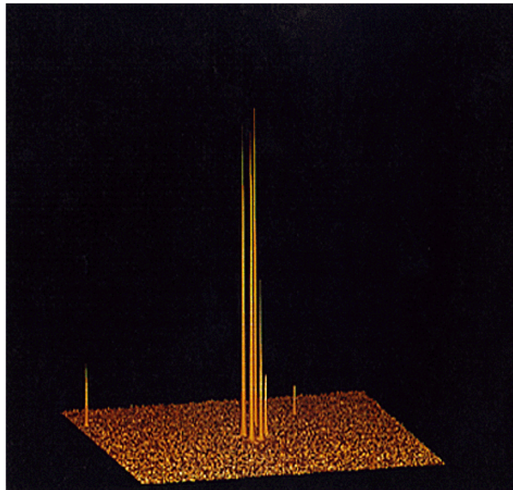
3-D representation of Chandra simulation
