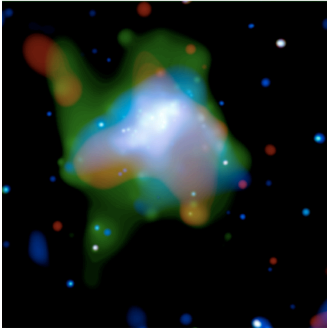
X-ray
