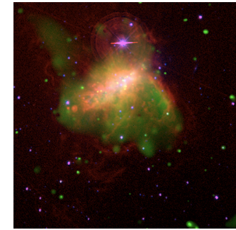
Optical/X-ray
