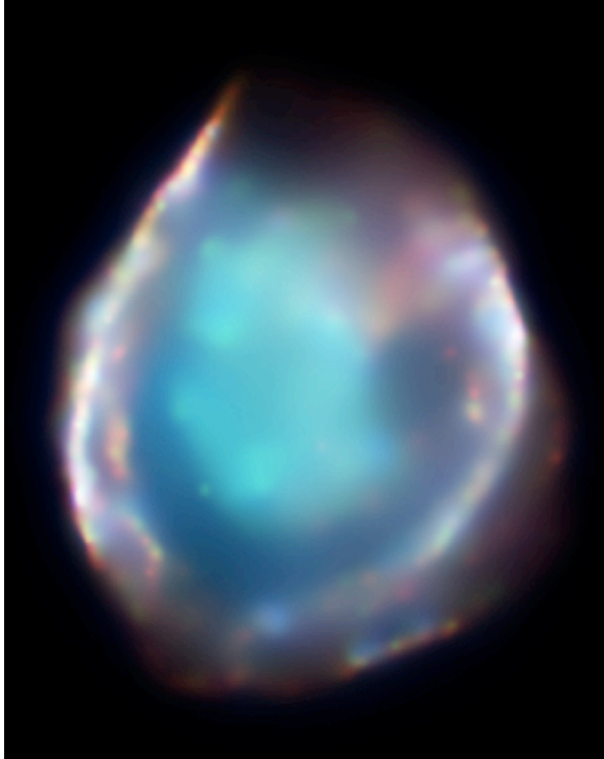
X-ray
