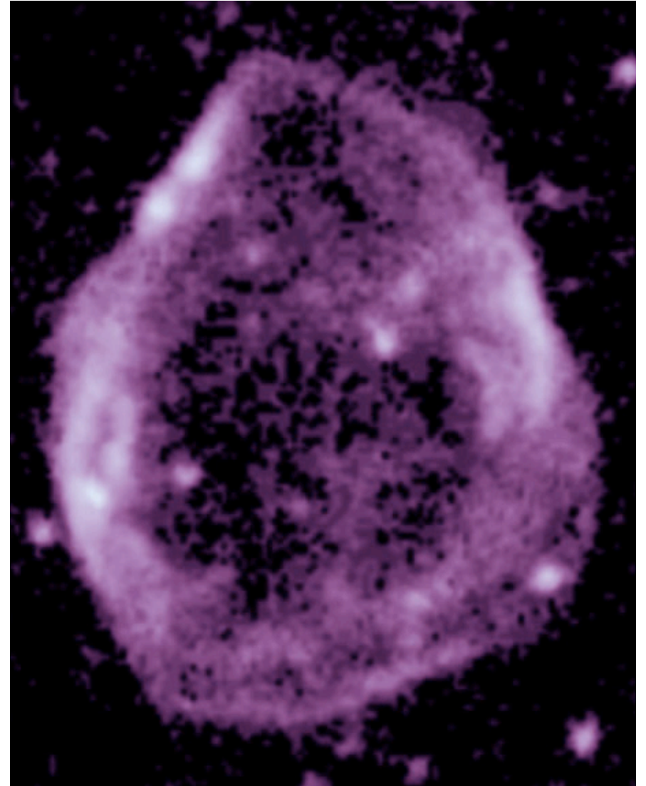
Optical (H-Alpha)
