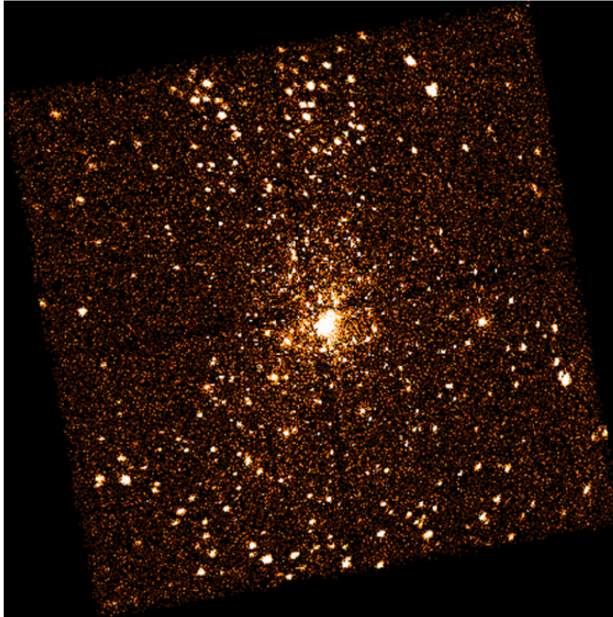
Orion Nebula, X-ray
